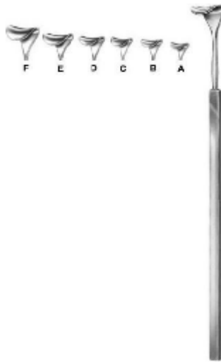
Cushing UE-5-926-08 Saddle Hook 20.5 cm 8 mm wide, 20.5 cm 10 mm wide, 20.5 cm 12 mm wide, 20.5 cm 14 mm wide, 20.5 cm 16 mm wide, 20.5 cm 18 mm wide,
